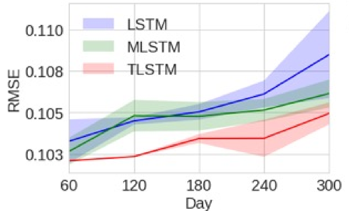
Climate dataset
