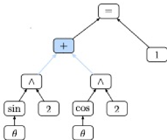
Choose Node
