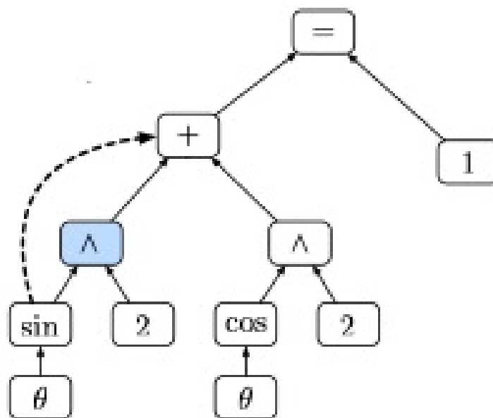
Shrink Node
