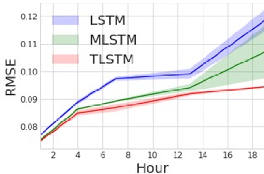
Traffic dataset
