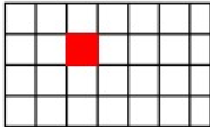
Pairwise correlations
